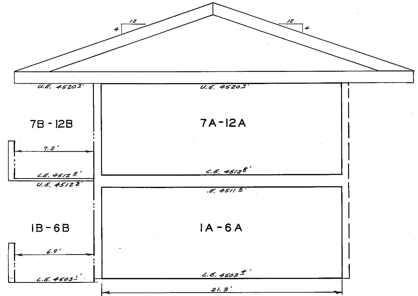
UNITS IA - 12A SCALE : 1" = 4'
