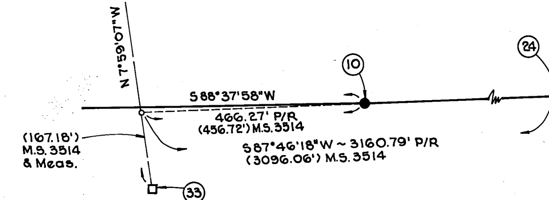
DETAIL 1" = 200'
