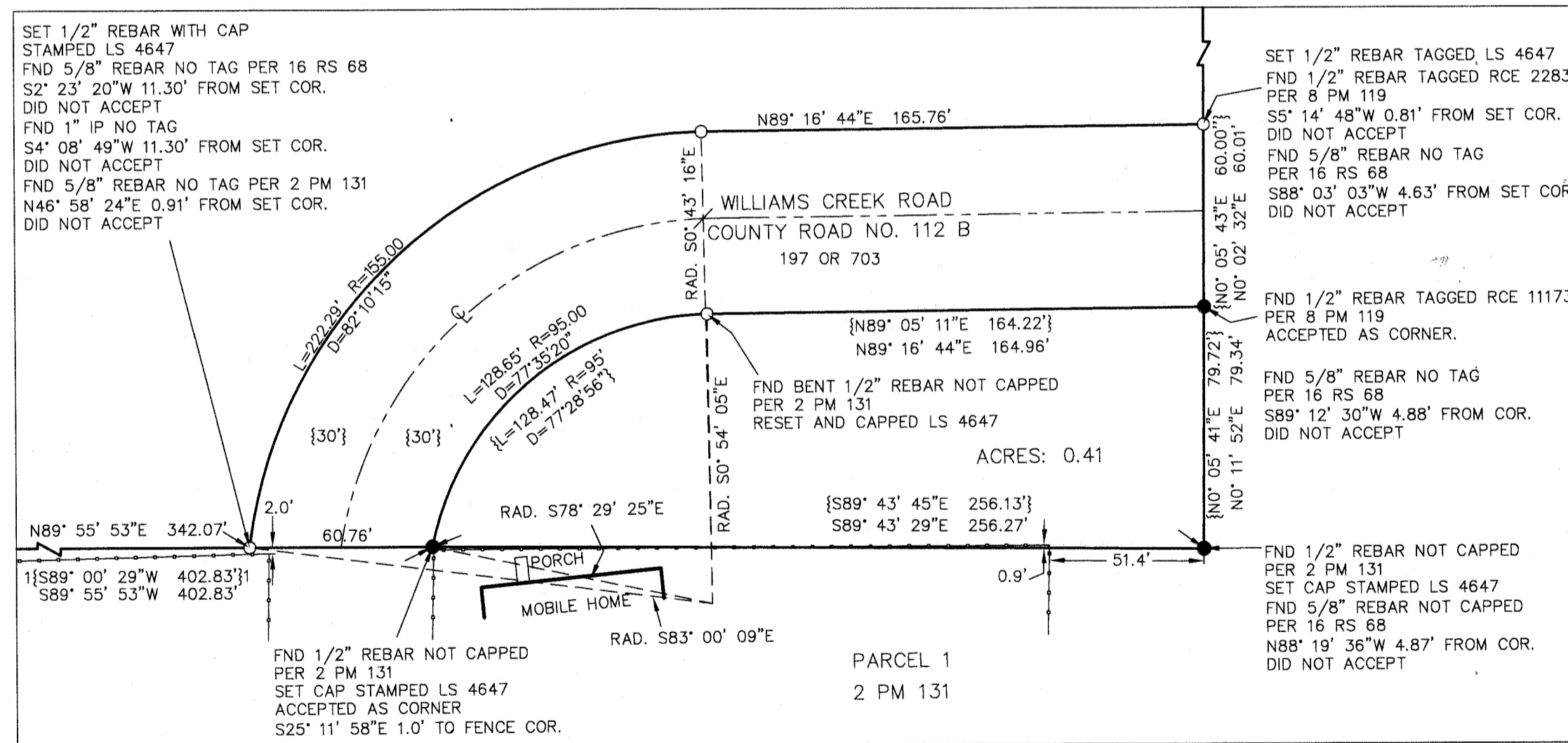
DETAIL C NOT TO SCALE
