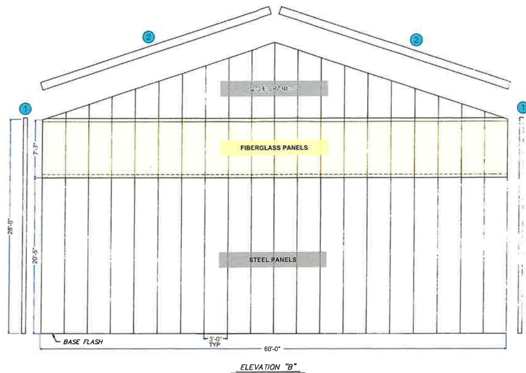
ELEVATION "B"
